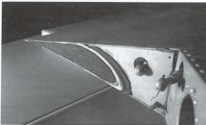
Perhaps it was Professor Joseph Cornish and his test pilot, Sean Roberts, who glued these thin sections of dark felt onto the root ends of the flaps when they evaluated Sisu 1A N1100Z at Mississippi State University in 1963. By closing this thin gap between the flap and the fuselage, they eliminated another source of performance-robbing drag. (Credit: Mark Avino/SPS NASM)
