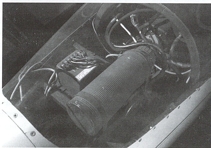
This ribbed cylinder is the air reservoir that is attached to the variometer installed in Parker’s Sisu 1A. It is insulated to prevent false readings due to changes in temperature. (Credit: Mark Avino/SPS NASM)
