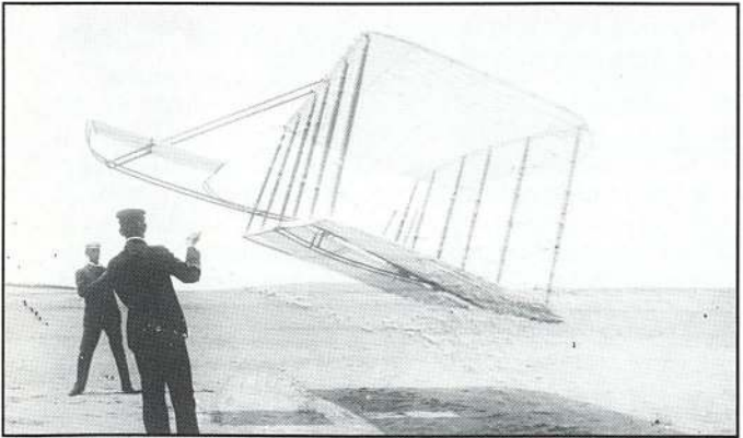
The Wright's second glider, the 1901, being flown as a kite. It had a moveable forward elevator but no rudder. Turns were made by "warping" or twisting the wings.
